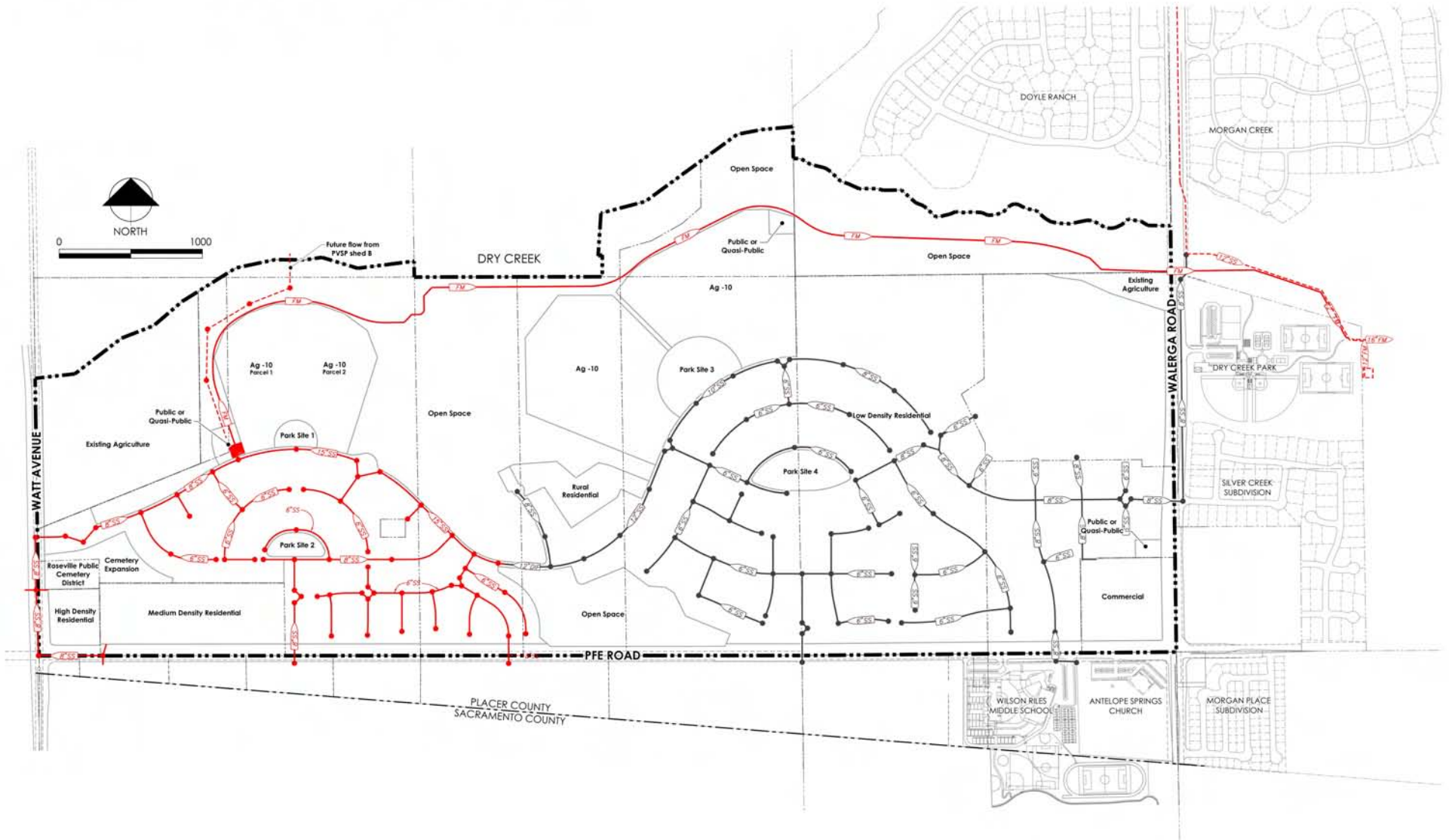
FIGURE 7.5 WASTEWATER ALTERNATIVE 3
