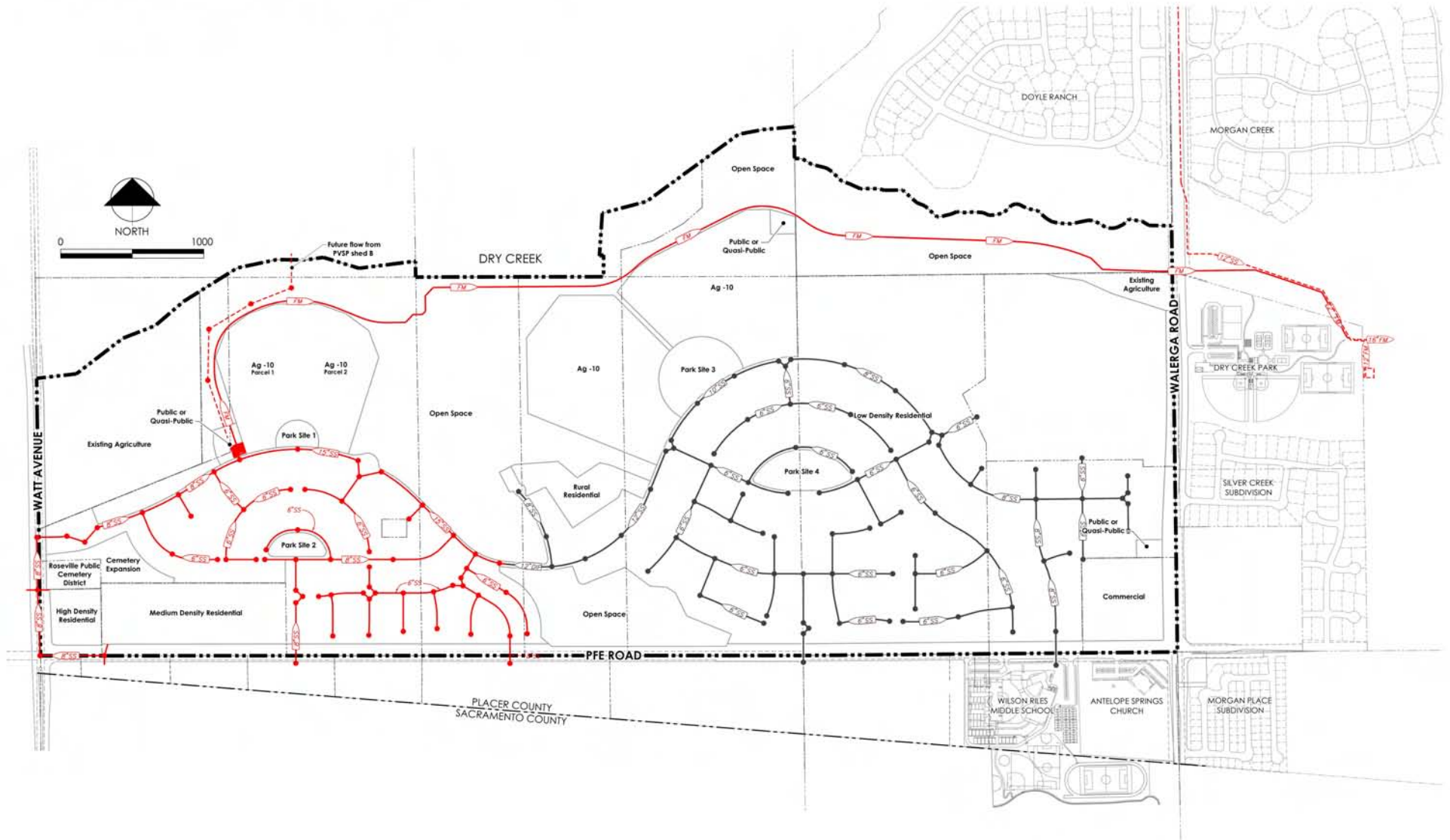
FIGURE 7.3 WASTEWATER ALTERNATIVE 1
