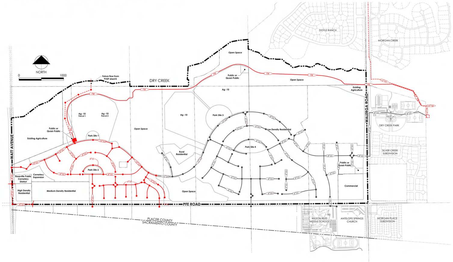
FIGURE 7.4 WASTEWATER ALTERNATIVE 2
